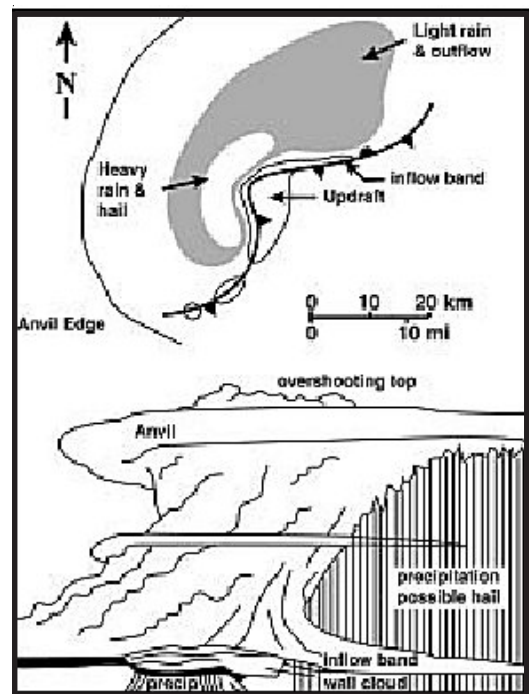
Figure 3-5. Typical High-Precipitation (HP) Supercell. These supercells develop in deep, moist layers with high moisture values.
