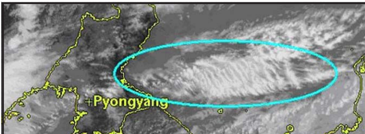
Figure 2-55. Example of Transverse Waves.
