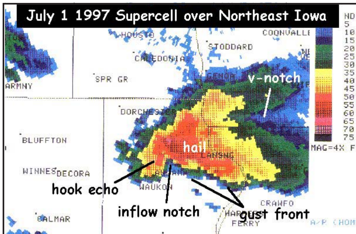
Figure 3-14. Supercell Example.
