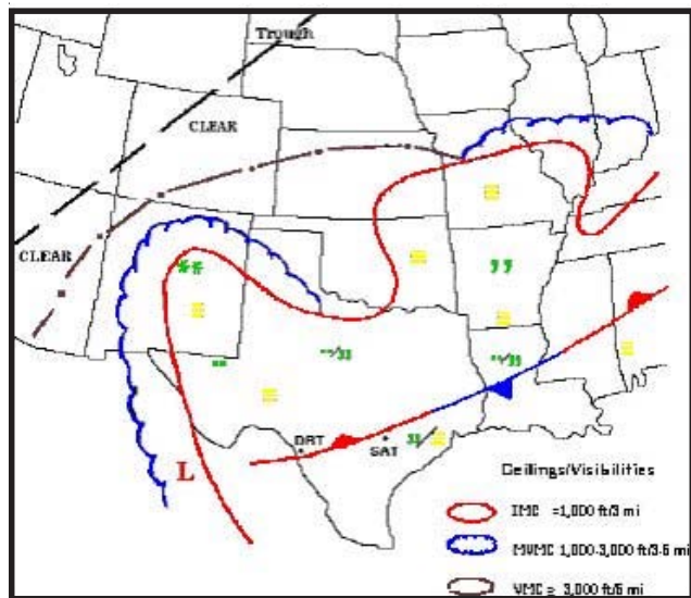
Figure 2-18. Nephanalysis Example.
