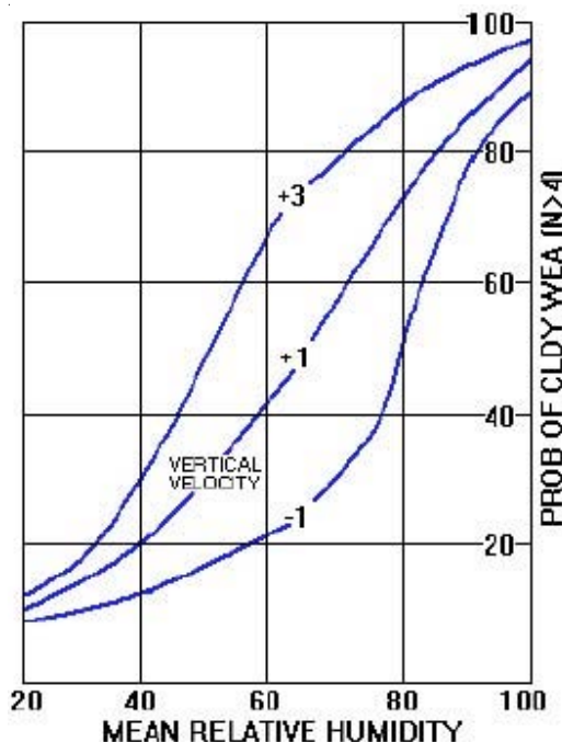
Figure 2-25. RH and OVV Graph. Probability of a ceiling based on RH and OVV values.
