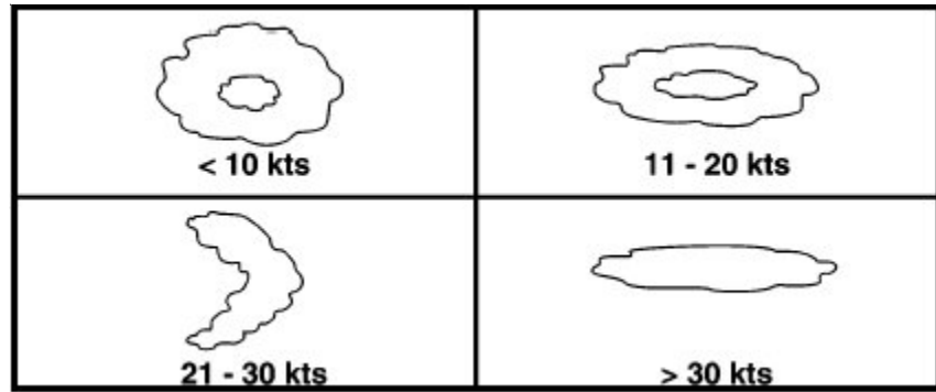
Figure 1-19. Open-Cell Cumulus Shapes. These formations are associated with straight-line or cyclonic flow.
