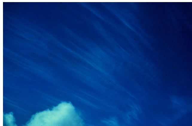
Figure 2-13. Cirrus (H1).
