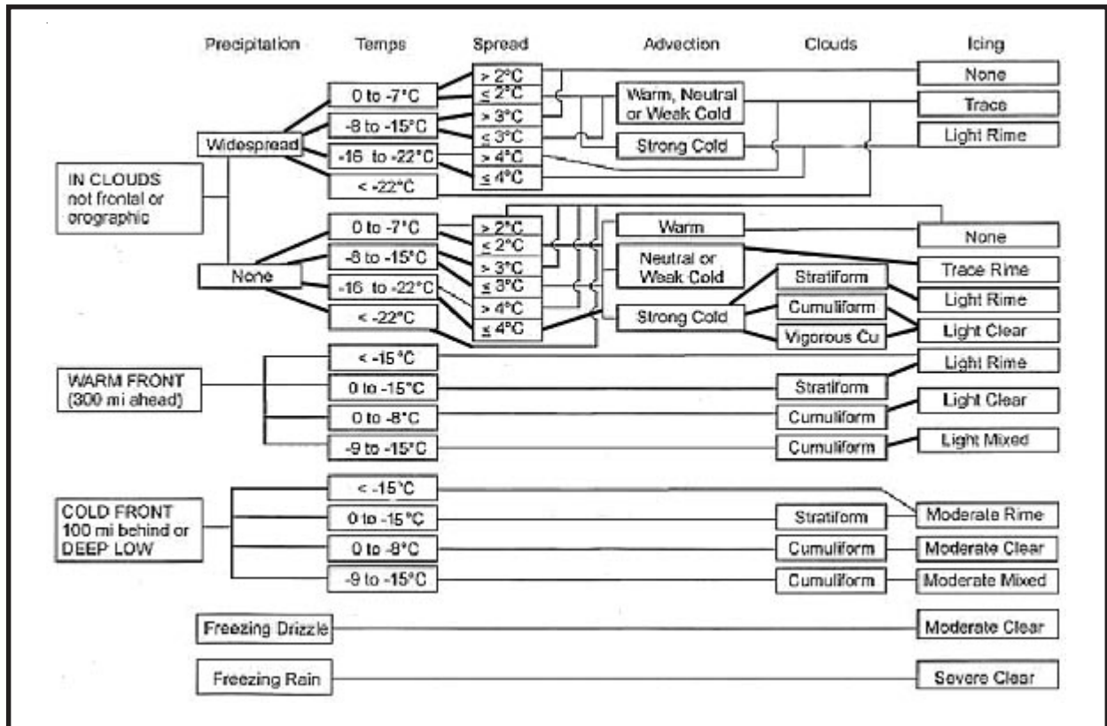
Figure 2-68. Icing Flowchart.
