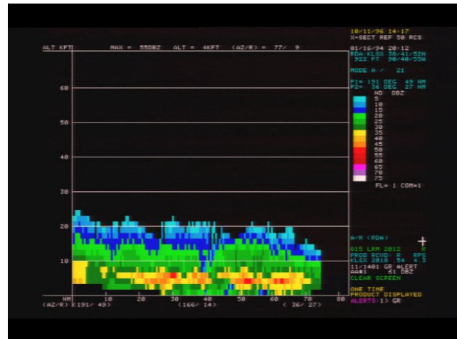
Figure 2-21. Reflectivity Cross-Section Product.
